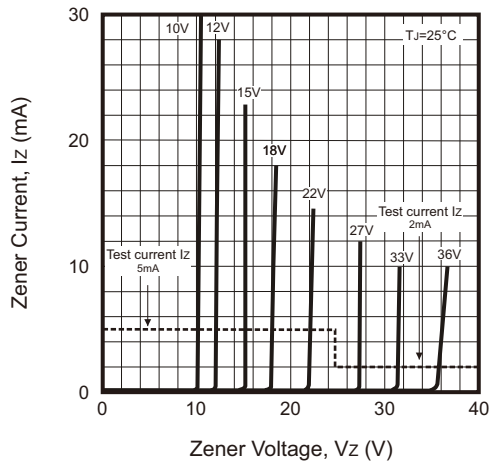
Fig.3 - Typical Zener Breakdown Characteristics
